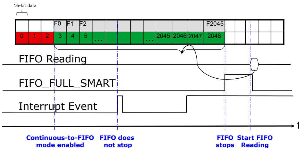
Figure 30. Continuous-to-FIFO mode
