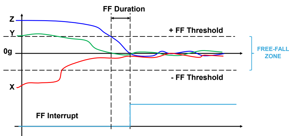
Figure 12. Free-fall interrupt
