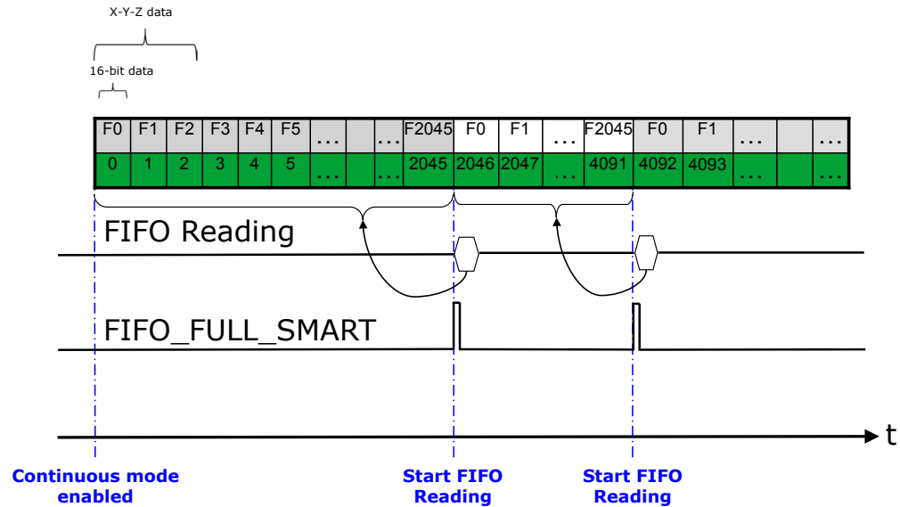
Figure 29. Continuous mode
