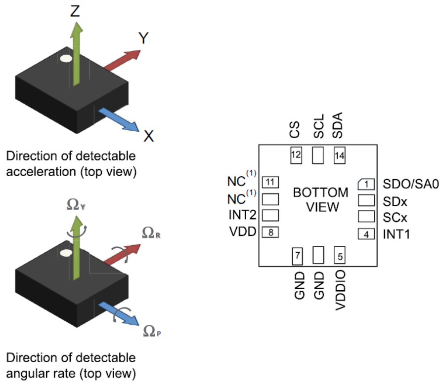
Figure 1. Pin connections
